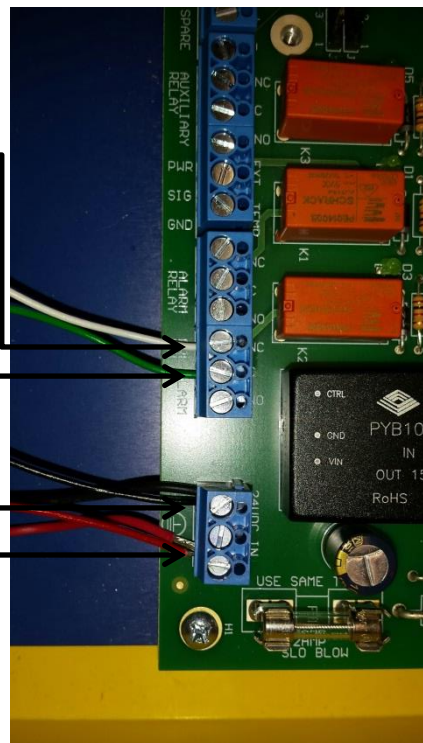
LBW-420-1 Relay connections
