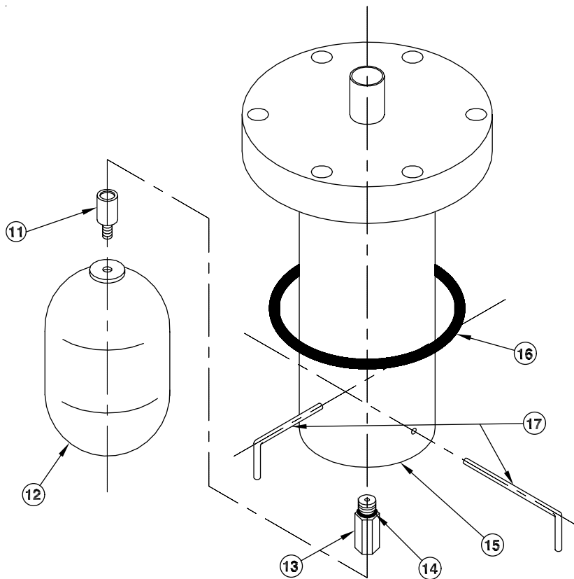
Purifier Vessel Cover and Float Ball Assemblies
