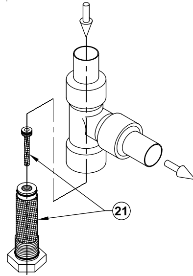
Strainer/Orifice (5a, 5b)
