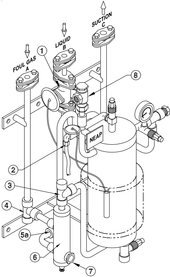
Left-Hand Side
