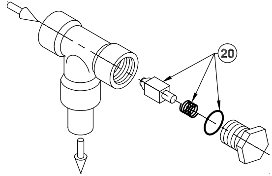
225 psid Check Valve (10)
