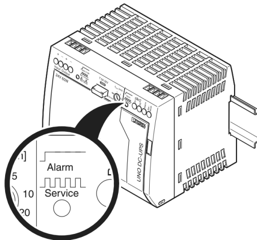
UPS LED Alarm Indicator - Red LED
