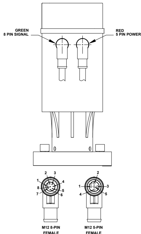
Power Connector - 5 Pin Red Cable
