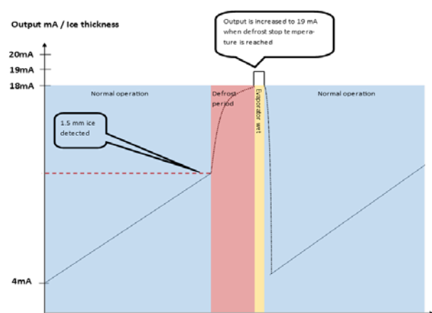
Graphical view of a typical sequence on an air cooler
