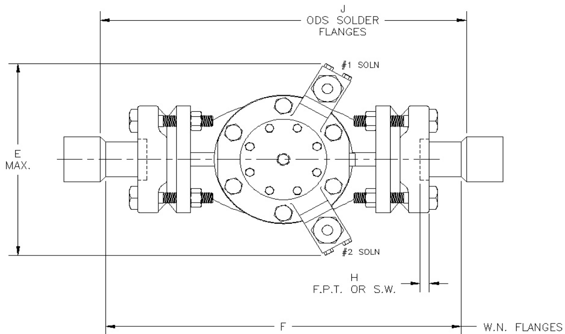
Fig. 4: CK-2D Dimensions
