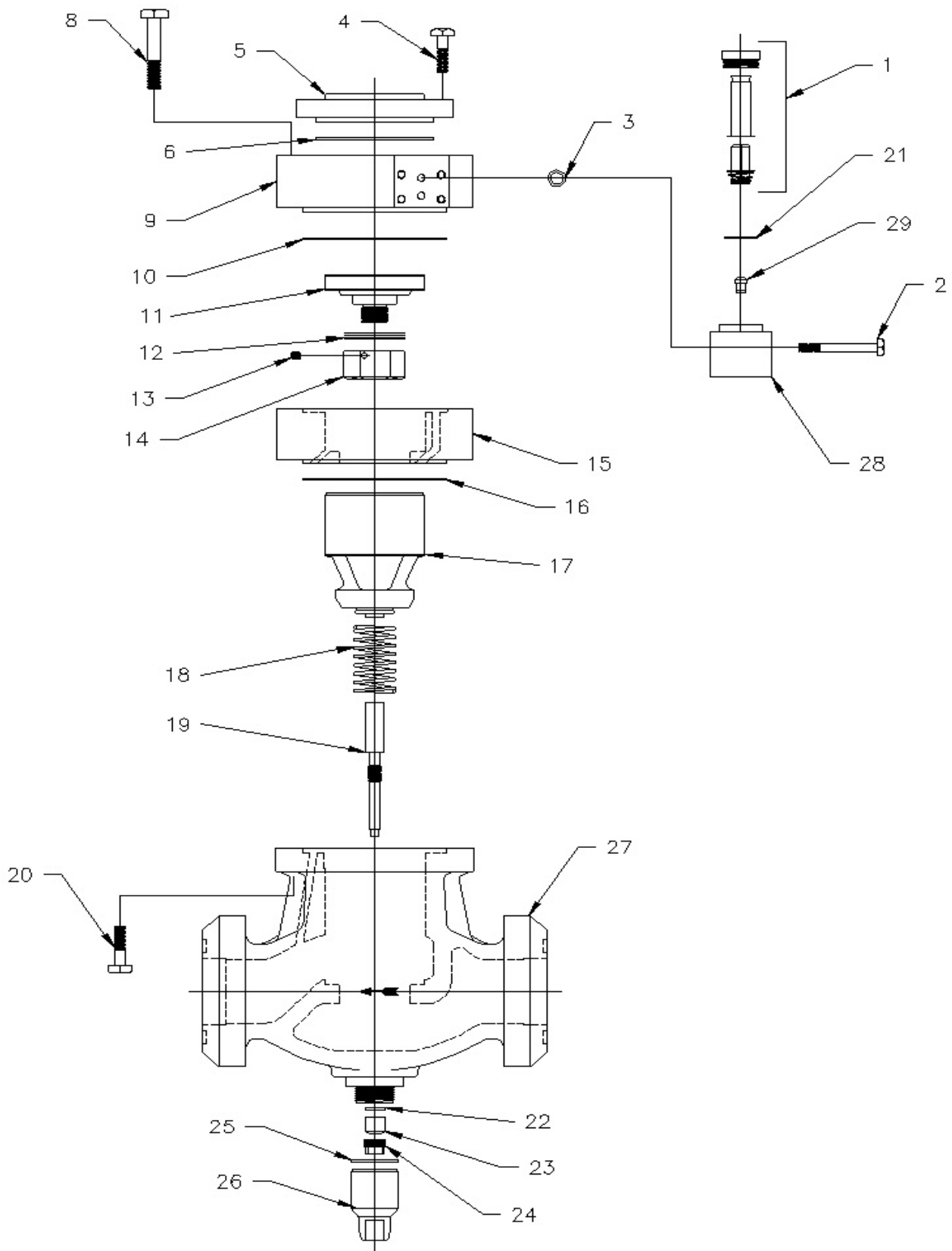
Fig. 3: CK-2D Exploded
