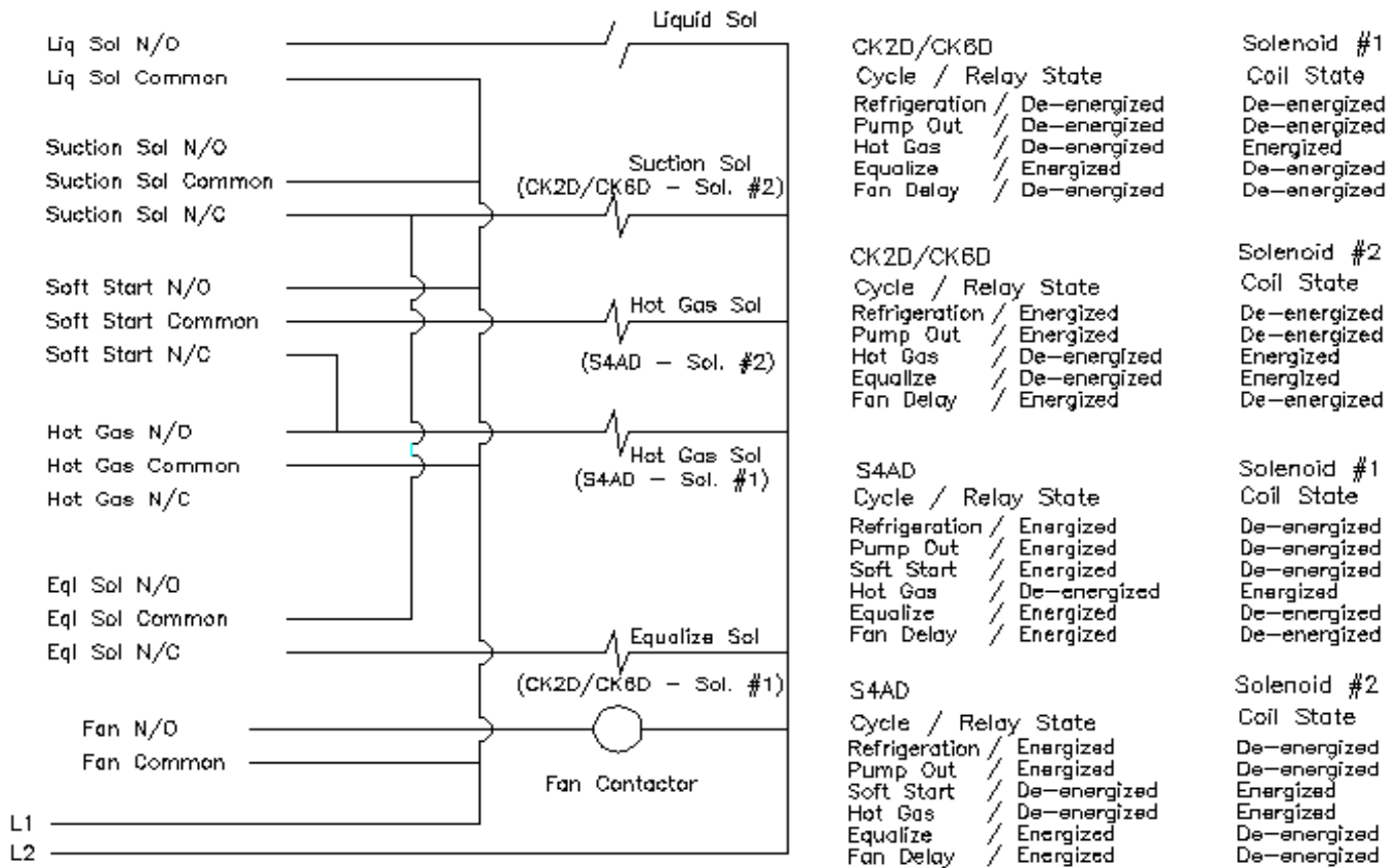
Fig. 5: R/S Defrost Controller Wiring Diagram CK-2D/CK-6D Line Equalization, S4AD Soft Start
