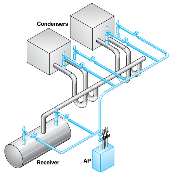
AUTO-PURGER AP application with six purge points.
