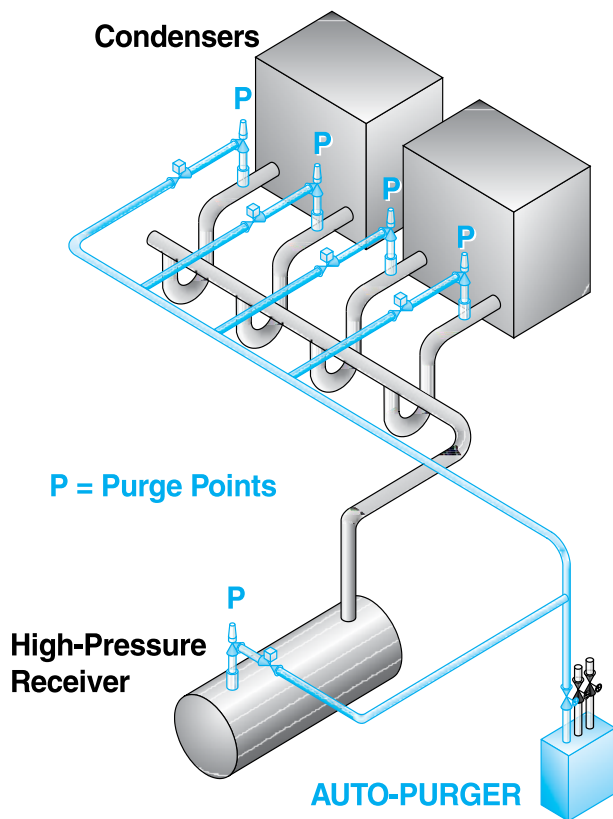
Multipoint purging.
