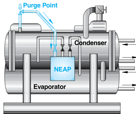
AUTO-PURGER NEAP installed on a skidded chiller package for use in hazardous atmospheres.
