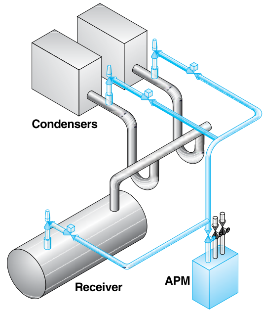
AUTO-PURGER APM application using three purge points.
